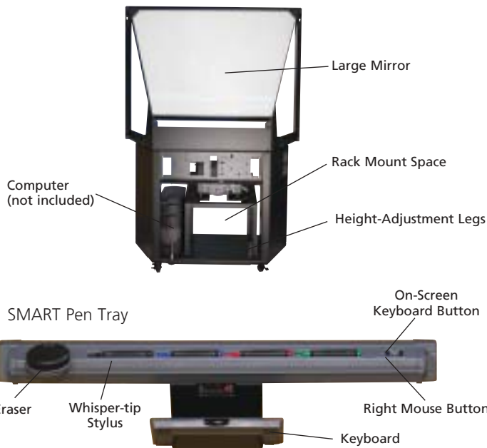
SMART Mirror Stand – Back View
